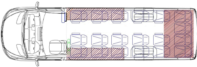
Attachment 2 - Seats - Scheme
